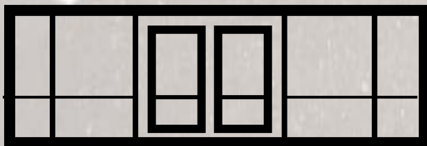
HT5 with 4 mullens positioned to accept 2 x 430 window cassettes, 2 x 880 window cassettes 1 x 880 door cassette.
